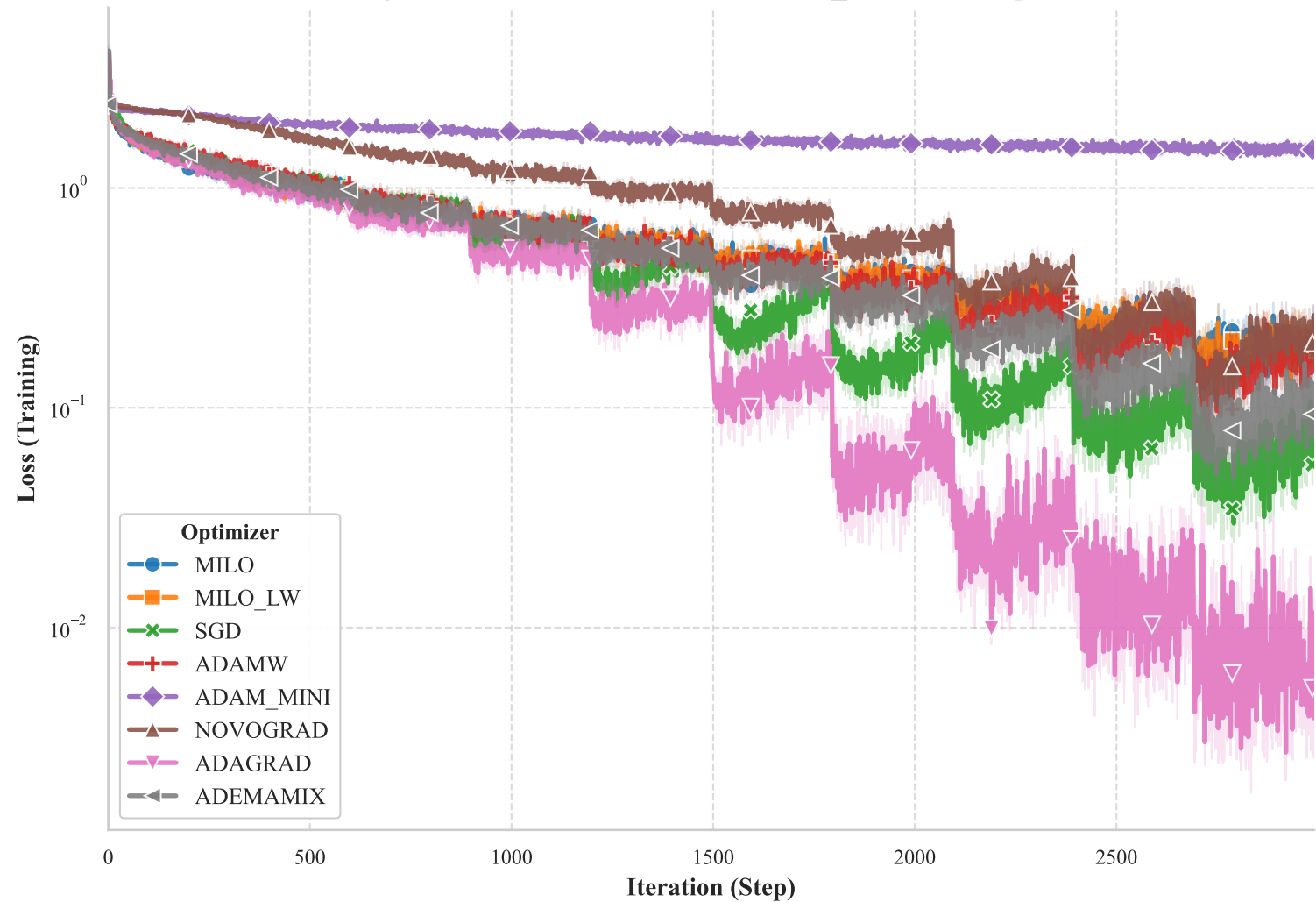
Training Loss vs. Iteration for RESNET34_CIFAR10 Experiment
